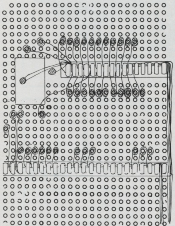
Figure 5: Detail of wiring on small board
